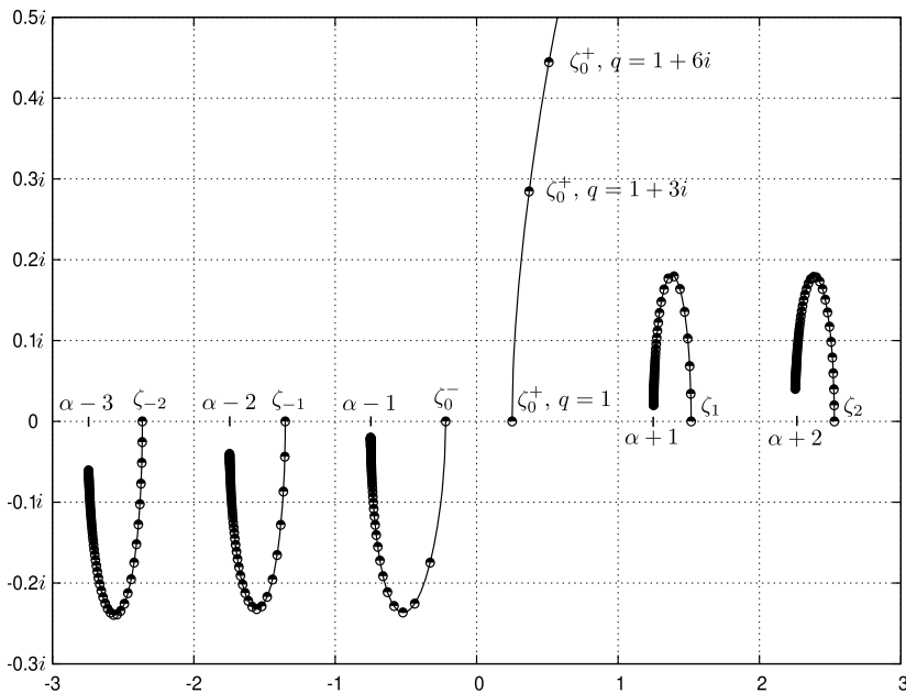
FIG. 2. The values of \zeta_0^\pm and \zeta_n for q \in [1, 1 + 200i] .
