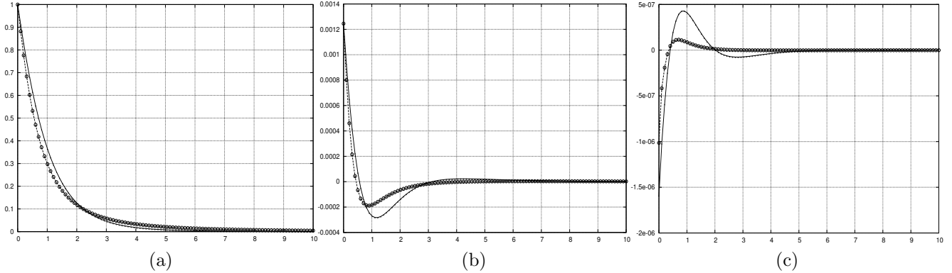
Figure 1: (a) The density of the exponential functional I_1 with N = 400 (the benchmark). (b) The error with N = 20 (no correction). (c) The error with N = 20 (with correction term). Solid line (resp. circles) represent parameter set I (resp. II).
